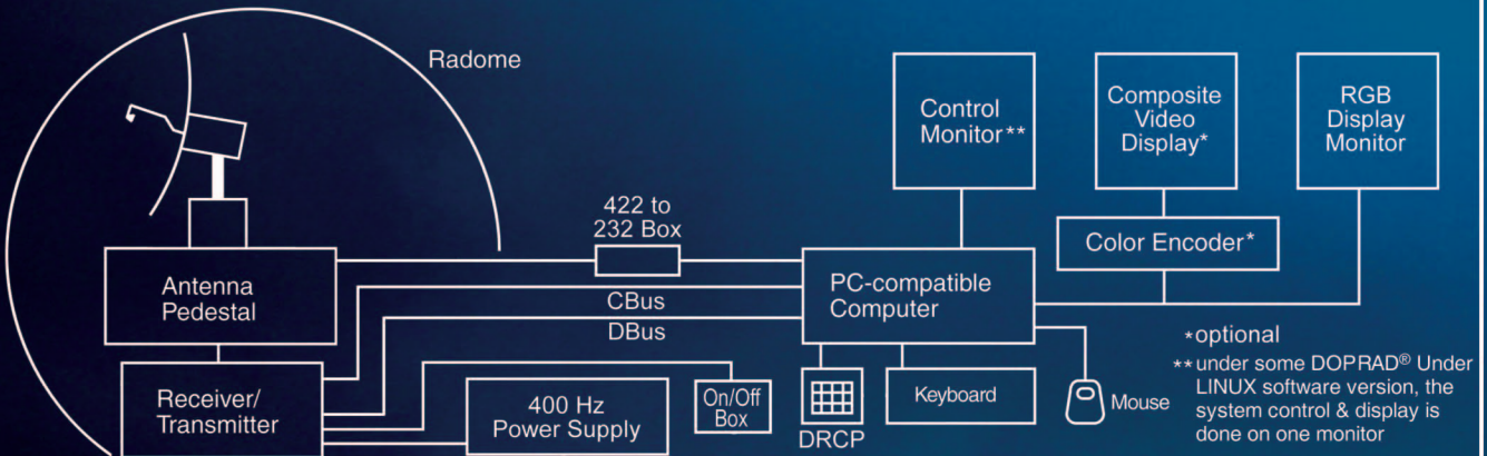
DOPRAD®/ Collins 6.33' or 8.33' System Diagram
