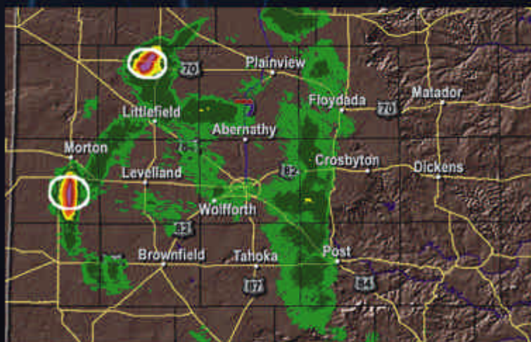
Mesocyclone Example
