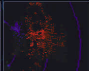
Microburst Example
