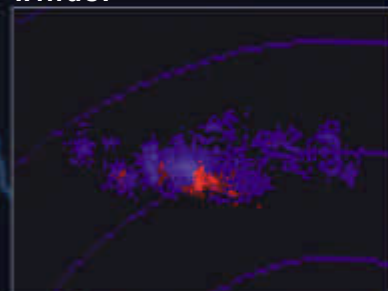
Mesocyclone Example
